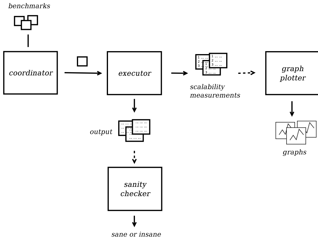
Figure 2: The architecture of bencherl.
