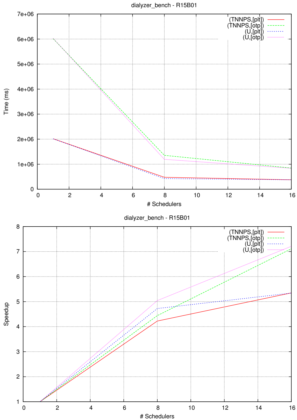
Figure 7: Running the dialyzer_bench benchmark, in order to build a PLT and then analyze all the Erlang libraries, with Erlang/OTP R15B01 and different scheduler bind types (u and tnnps ).
