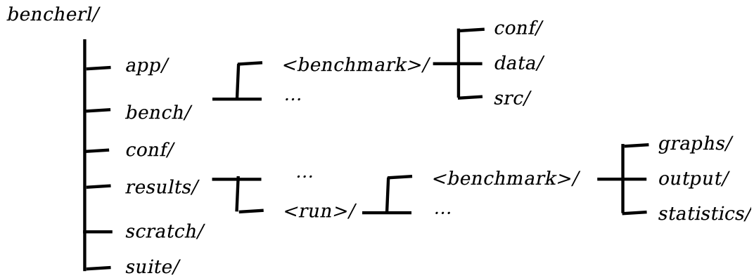
Figure 1: The current directory structure of bencheri .
